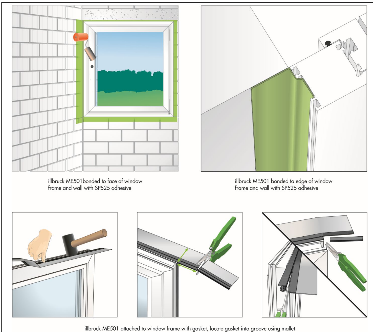
Figure 5 Installation of illbruck ME501 Duo Window Membrane HD with SP525 Adhesive or gasket
