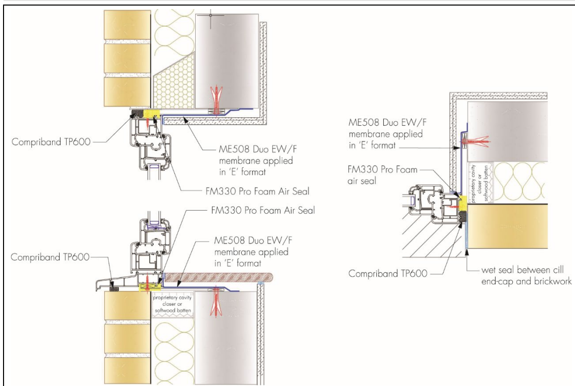
Figure 2 Typical installation detail
