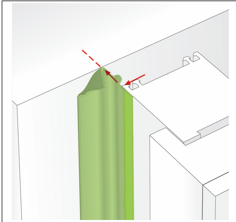
Figure 3 Application of illbruck ME508 Duo Membrane EW/F – 'E' format
