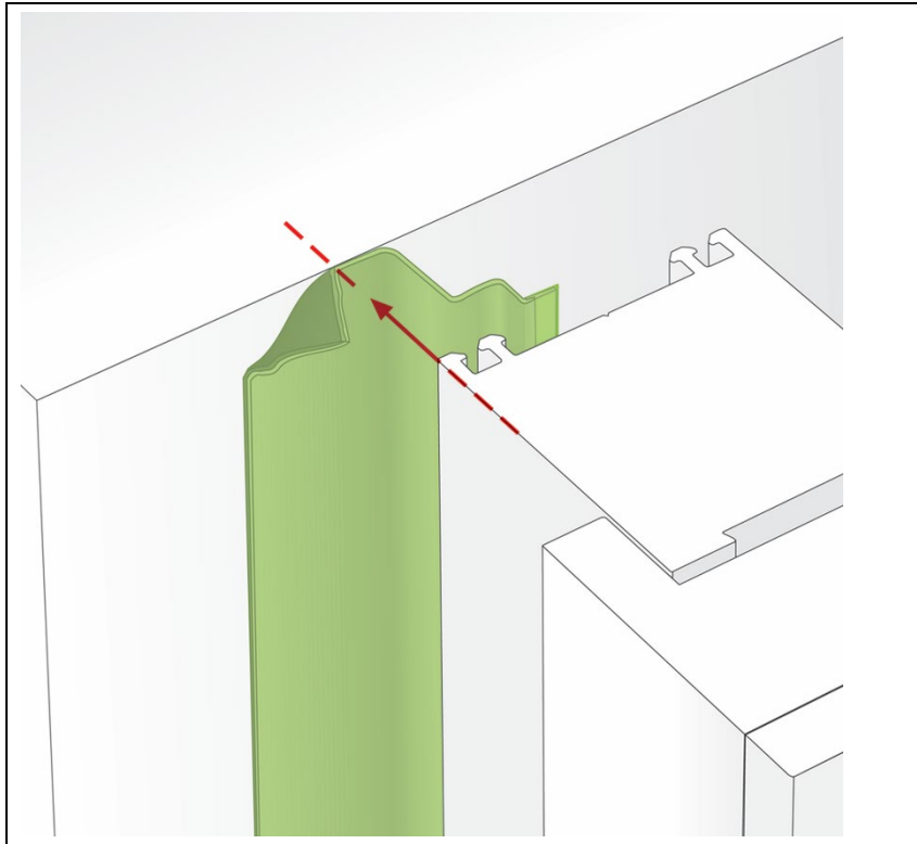
Figure 4 Application of illbruck ME508 Duo Membrane EW/F – 'W' format
